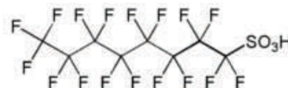
Perfluorooctanesulfonic Acid
